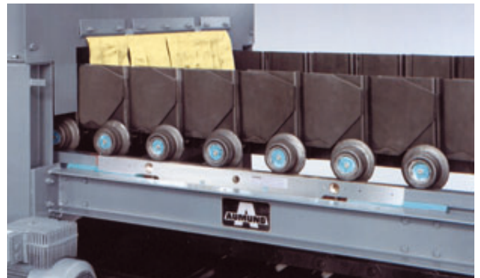
Weighing rail
