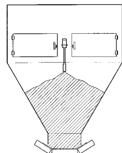
Samson™ Material Feeder starts on low level stops on high level
