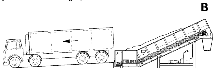
The complete truck contents transferred to the Samson™ Material Feeder body
