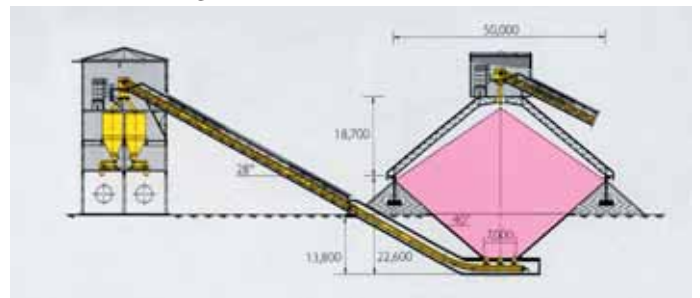
Circular Storage Hall with Earth Cone/without Central Column
