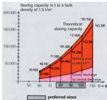
Storing Capacity Depending on the Storage Diameter
