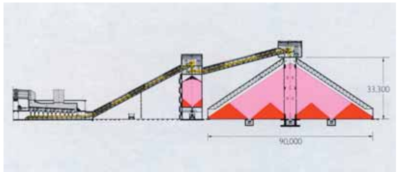
Covered Stockpile with Three Discharge Tunnels
