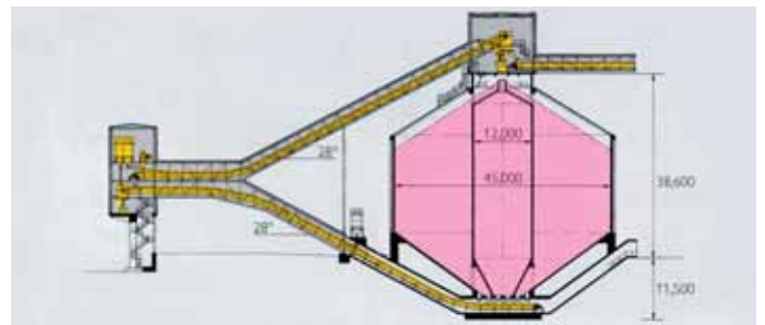
Circular Storage Hall with Internal Silo and Earth Cone
