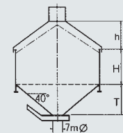
Circular storage hall with concrete cylinder, earth cone and steel roof without central column
