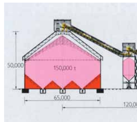
Circular Storage Hall
