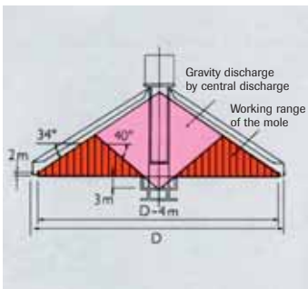
Working Range of the MOLEX™
