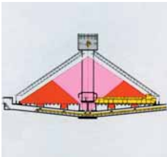
Covered Stockpile with MOLEX™ and Central Column
