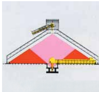
Covered Stockpile with MOLEX™ without Central Column
