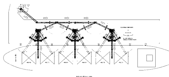
Telescopic Cascade Trimming Chute comprising a stack of inclined cones control the material flow velocity therefore prevent particulate separation controlling dust generation at the source
